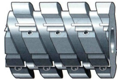
Figure 6 Reduced-noise cutter block
