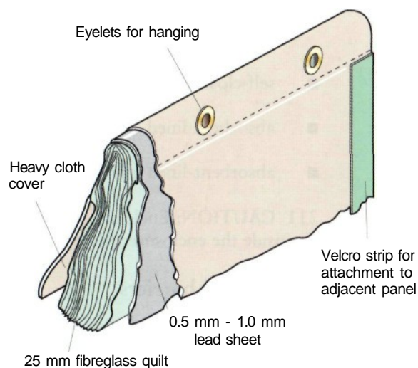
Figure 11 Example of construction of a hanging, flexible acoustic barrier
