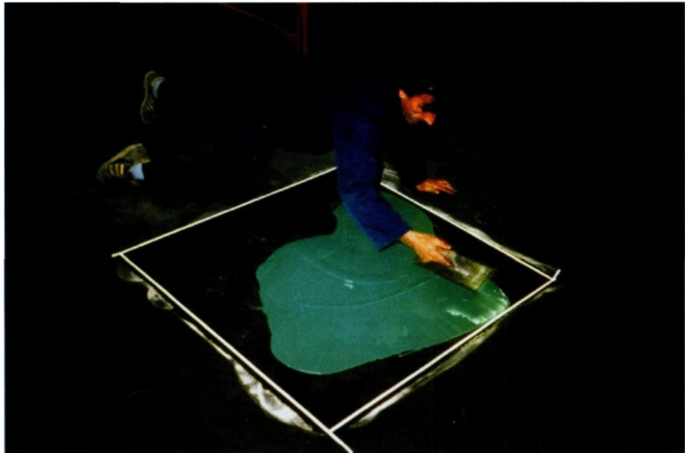
Figure 14 Damping compound being applied to metal decking
