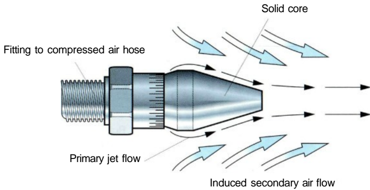
Figure 20 A low-noise (induced-flow) air nozzle
