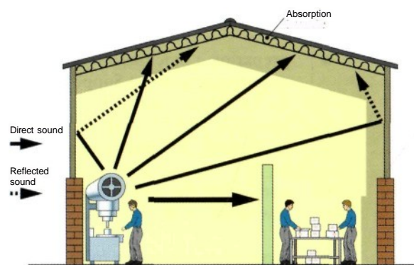
Added absorption to roof 'soaks' up reflected noise
